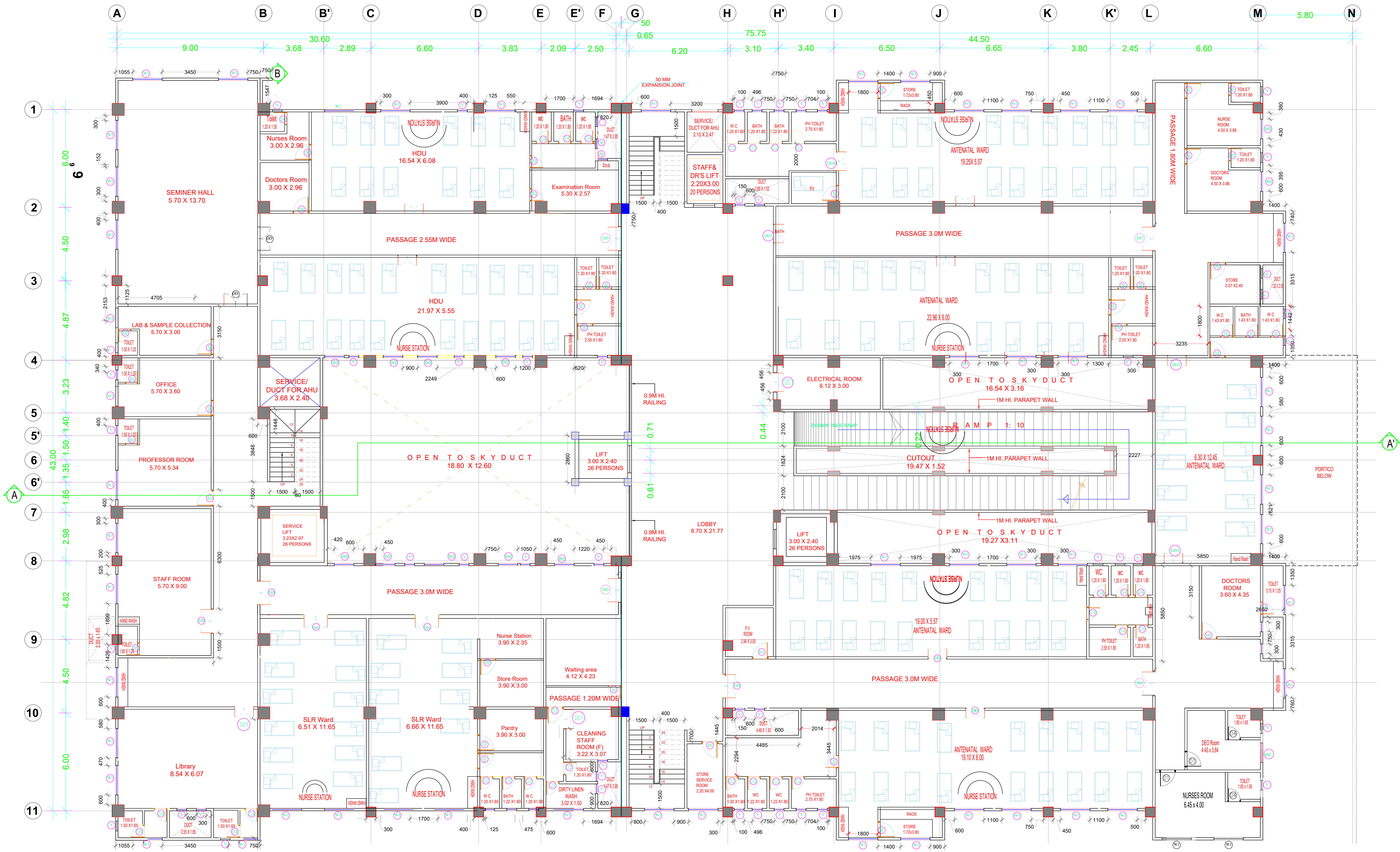
FIRST FLOOR PLAN
